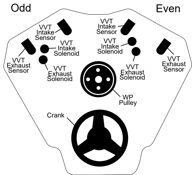
FRONT OF ENGINE Front View
